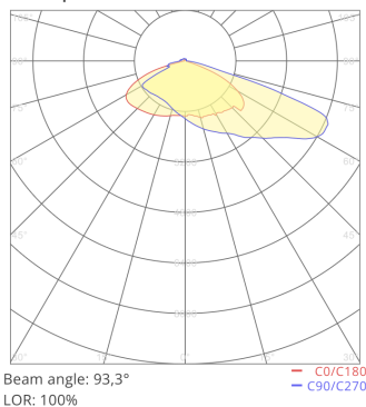
Polar plot
