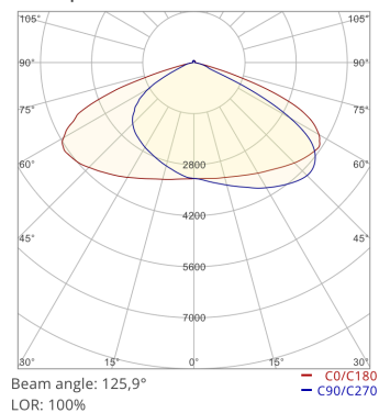
Polar plot
