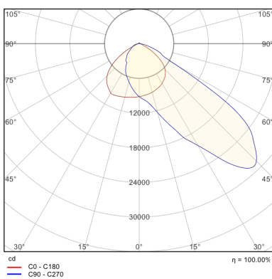
Polar light distribution diagram
