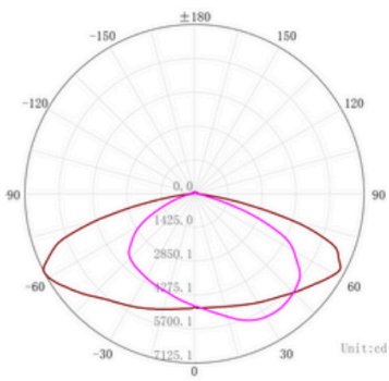
C Plane Distribution Diagram
