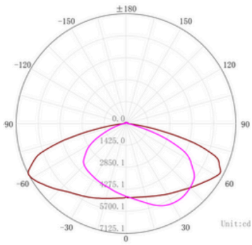
C Plane Distribution Diagram
